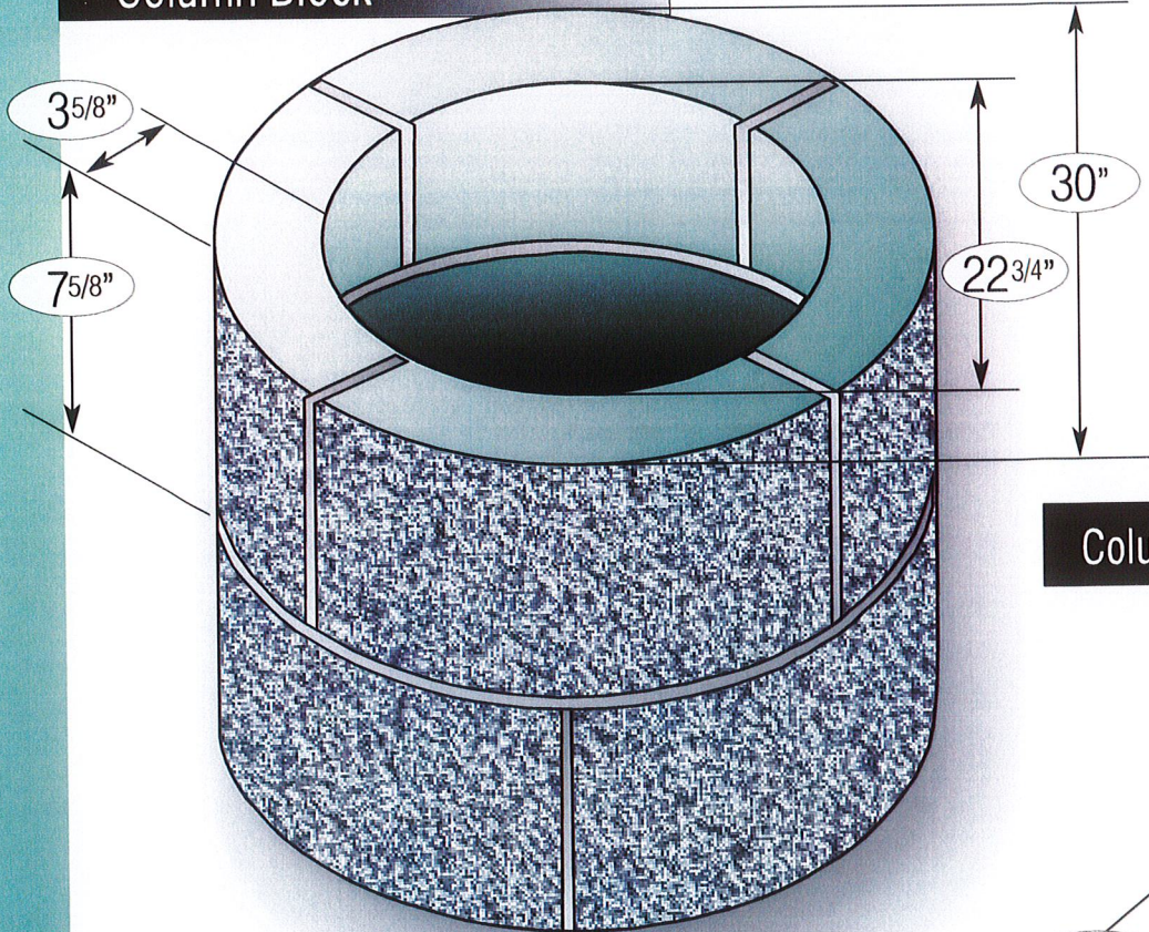
30" Column Block as Constructed
