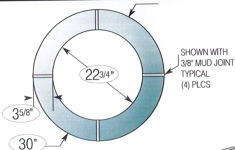
30" Column Block as Constructed
